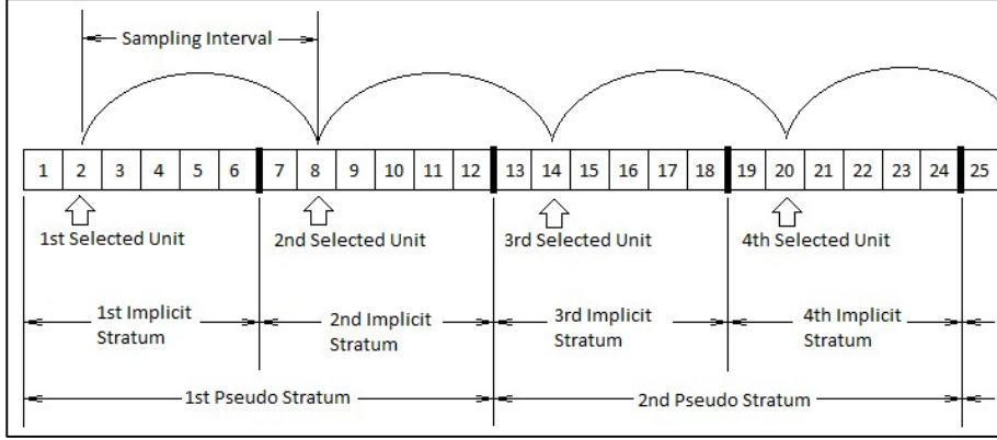
Figure 1: Representation of Systematic Random Sampling and Implicit Strata
