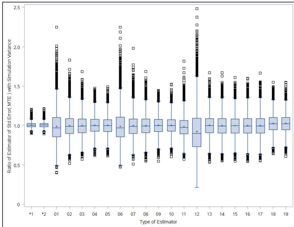
Figure 3: Distributions of the Ratio of the Standard Error Estimators – Random Sort Order
