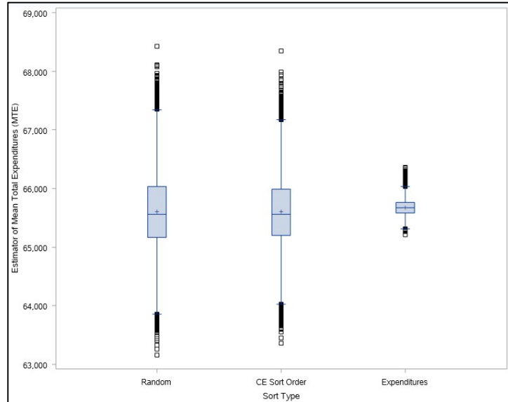
Figure 2: Distributions of the Estimators of Mean Total Expenditures for Varying Sort Orders
