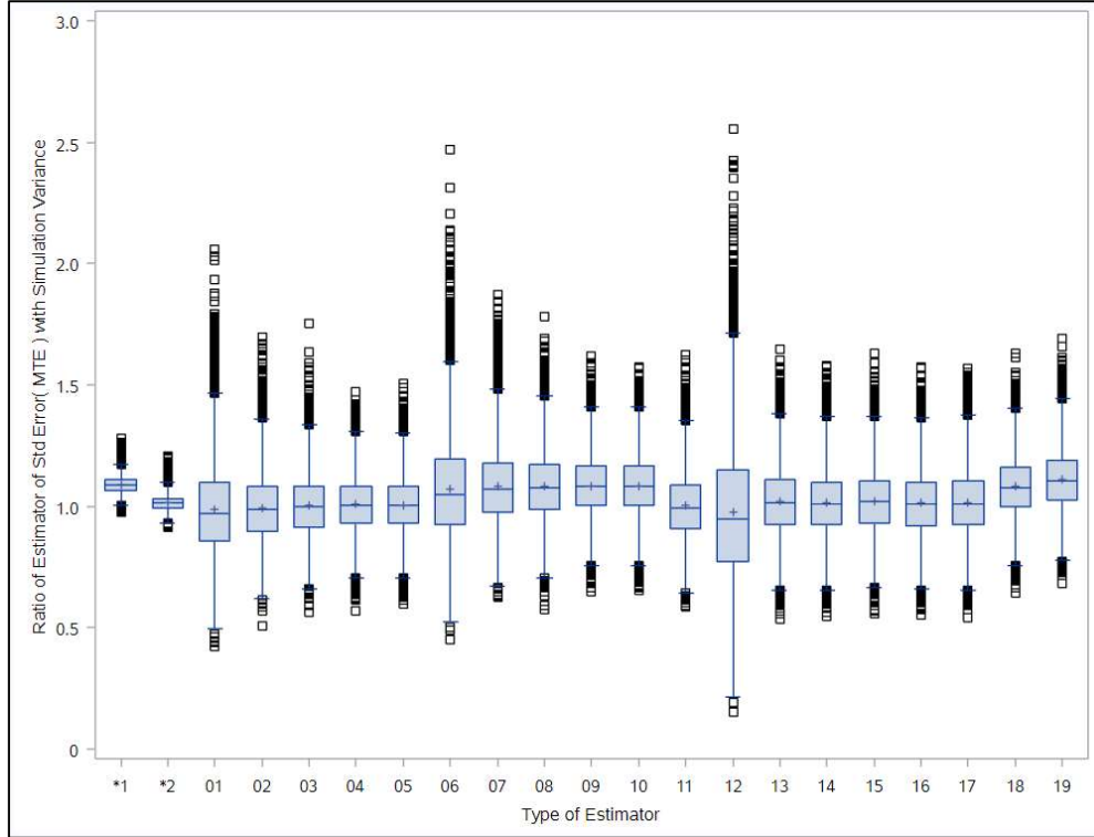
Figure 4: Distributions of the Ratio of the Standard Error Estimators – Approximate CE Sort Order
