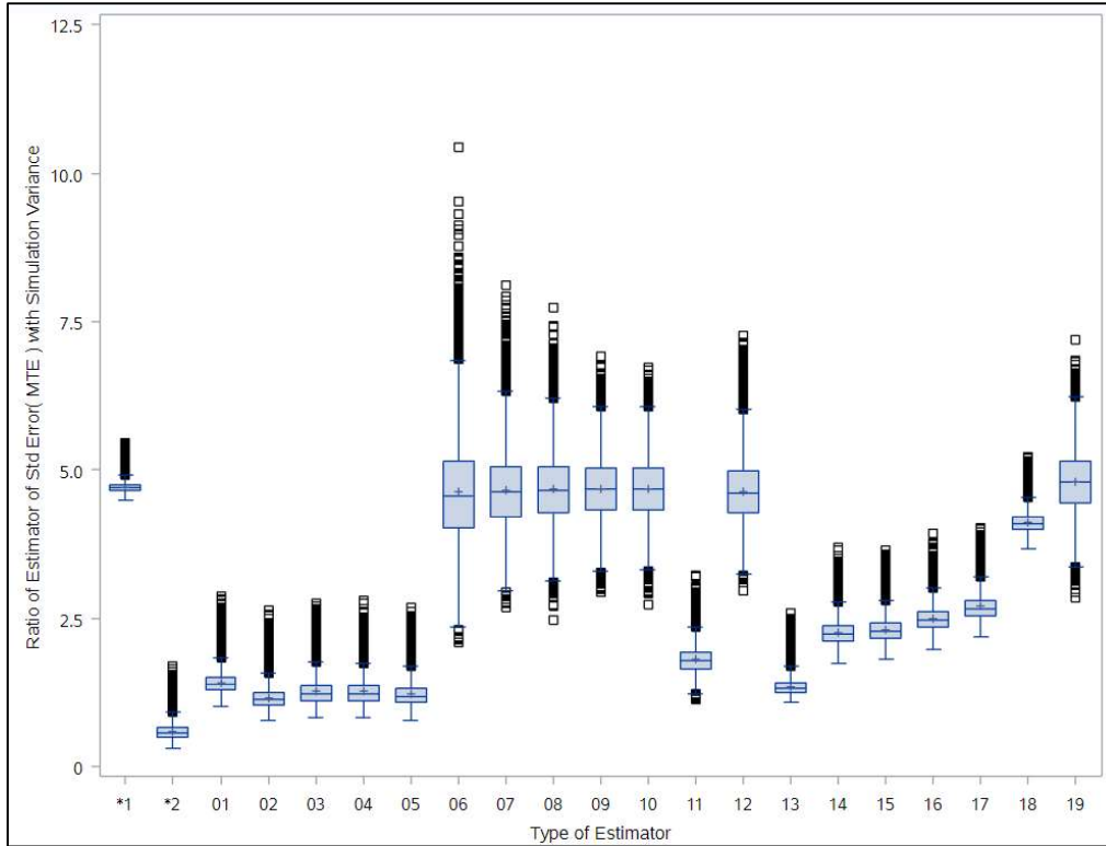
Figure 5: Distributions of the Ratio of the Standard Error Estimators – Sort by Expenditures
