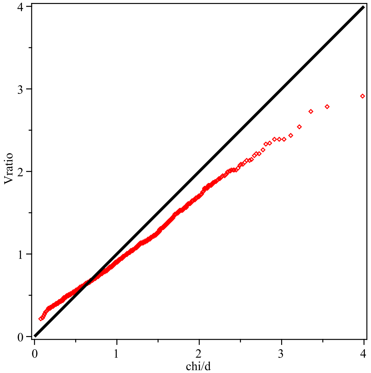
Figure 3: QQ plot of Vratio vs \chi^2_d/d (Chapter 90; Month=10; 1000 samples)
