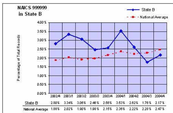
Figure 2: Percentage of Unclassified NAICS in State B in Comparison to the National Average of Unclassified
