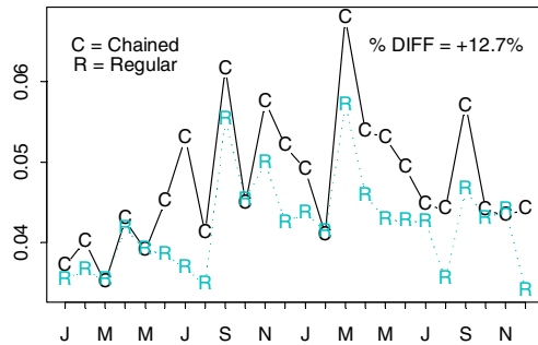
1-MO Standard Errors (Jan'00-Dec'01)
