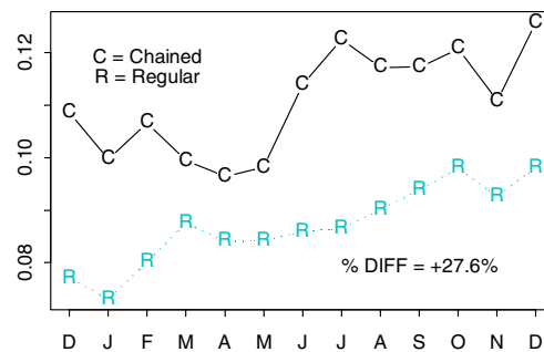
12-MO Standard Errors (Dec'00-Dec'01)
