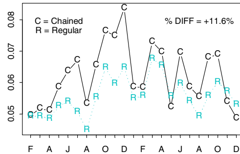
2-MO Standard Errors (Feb'00-Dec'01)
