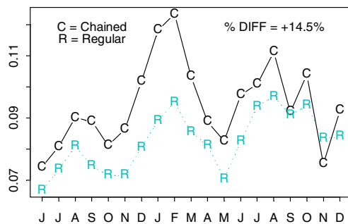
6-MO Standard Errors (Jun'00-Dec'01)
