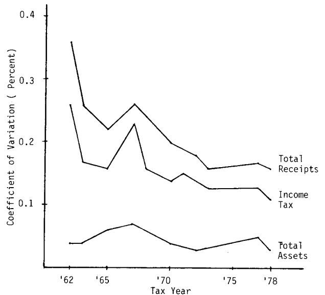
Figure C : Comparison of Coefficients of Variation for Selected Estimates
